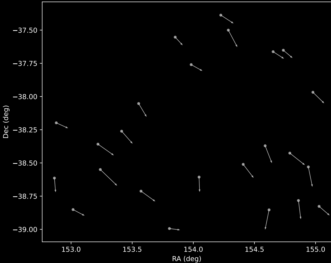
GALAH DR4 Cluster 15 Proper Motion Vectors (n=24)
