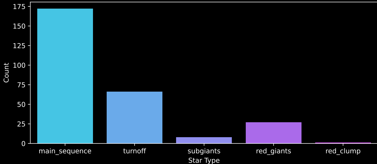
GALAH DR4 Field: [6917] Count plot of Star Type
