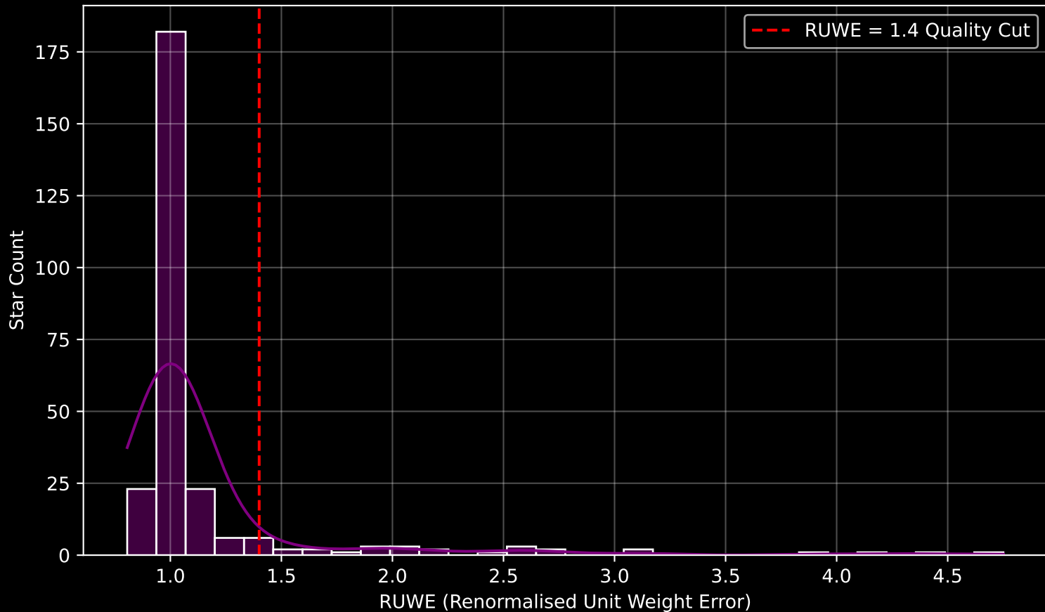
GALAH DR4 Field [6917] RUWE Distribution (n= 265)
