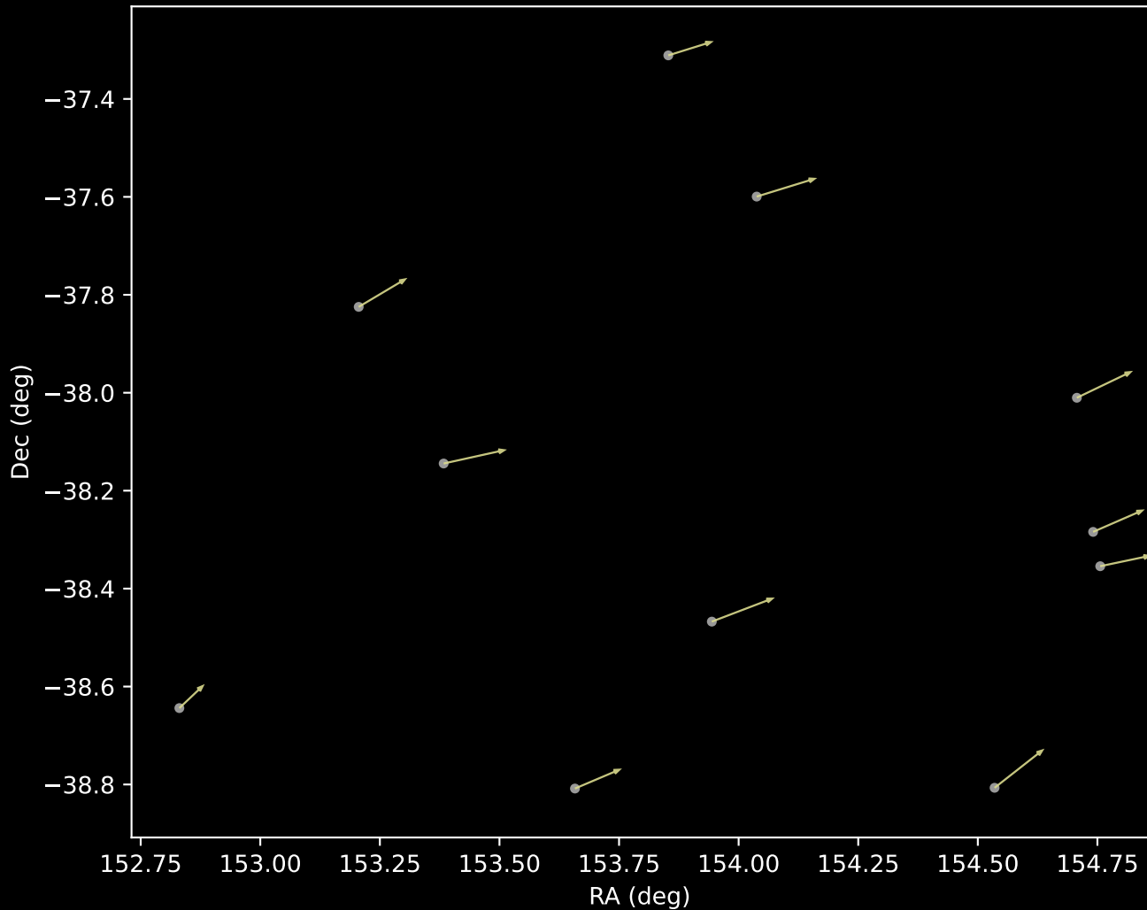
GALAH DR4 Cluster 17 Proper Motion Vectors (n=11)
