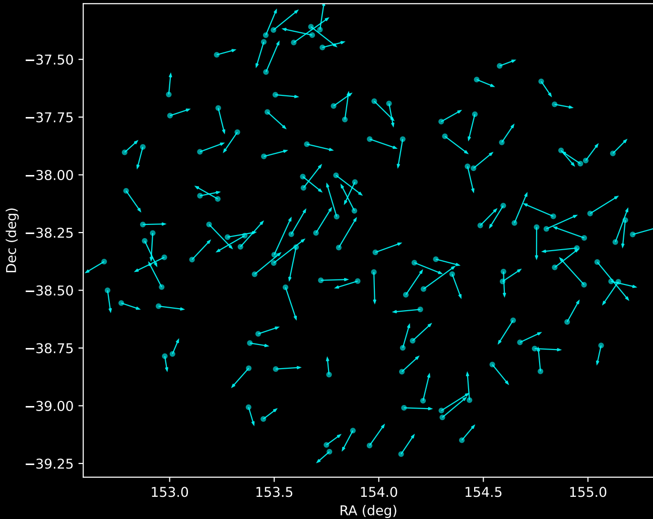
GALAH DR4 Noise Stream Proper Motion Vectors (n=131)
